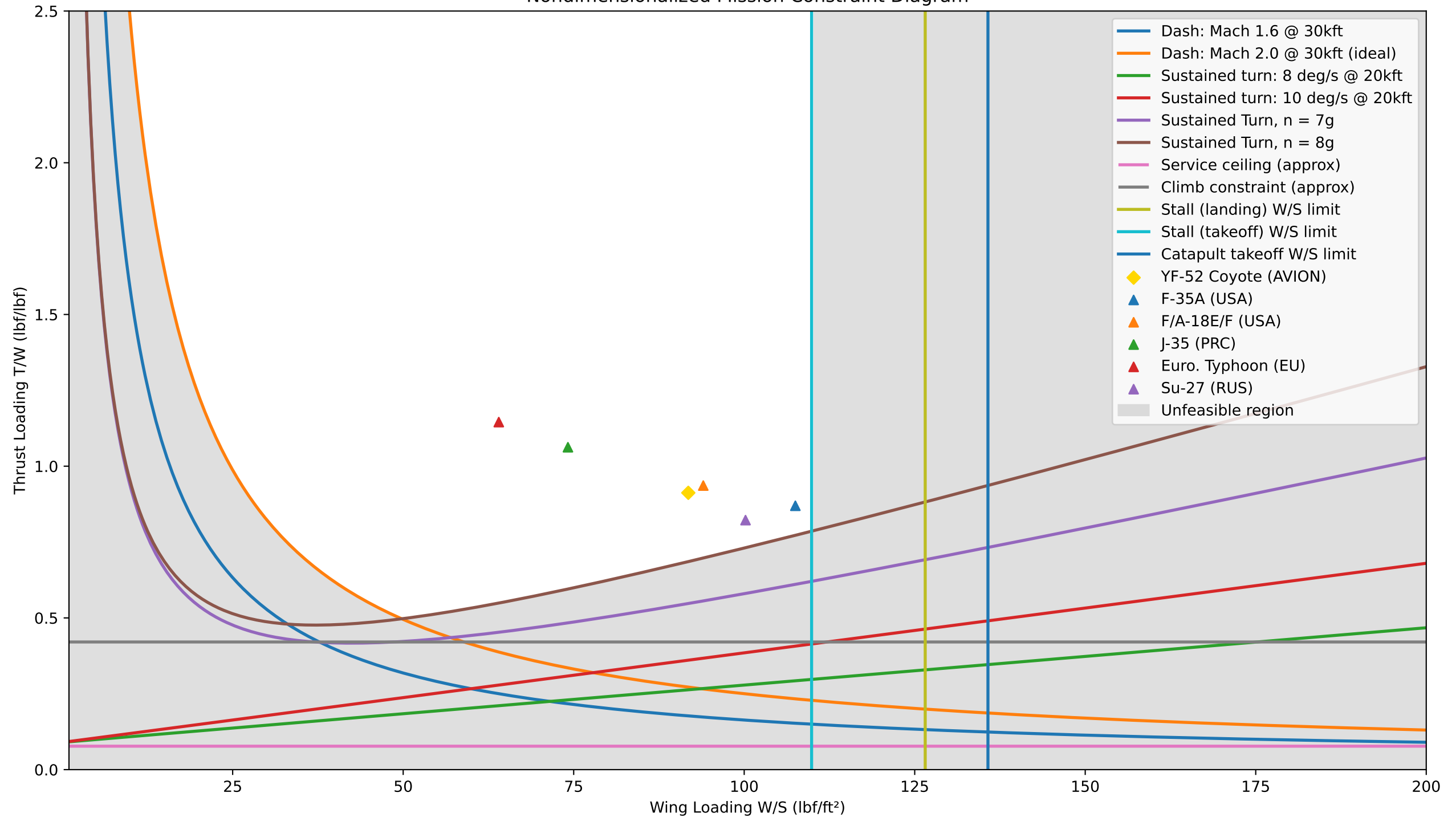
Nondimensionalized Mission Constraint Diagram
